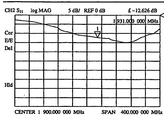
Return loss characteristic of the antenna in normal-use position near the user's head.
